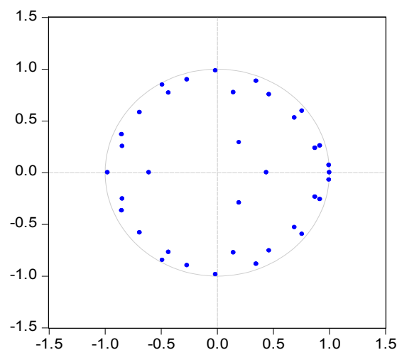
Figure A. Inverse roots of AR characteristic polynomial
